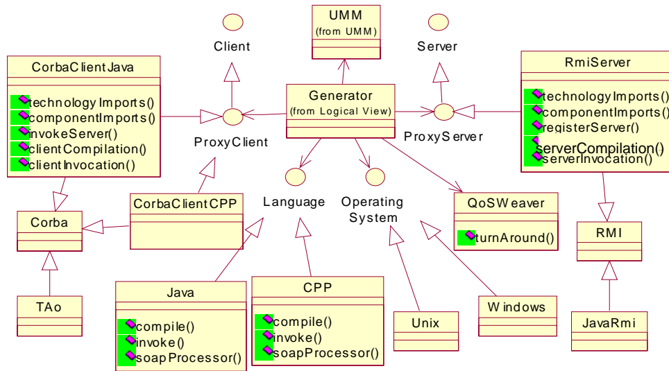
Figure. 3 The Glue/Wrapper Code Generator in Java
