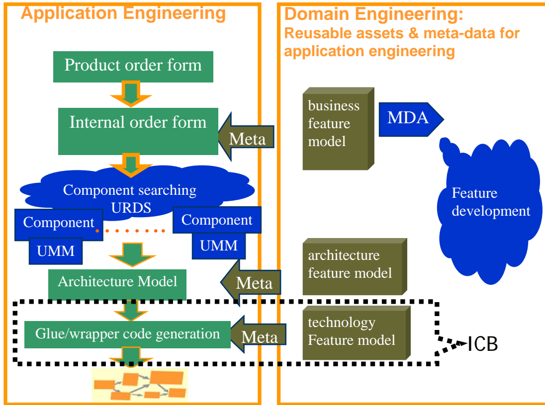
Figure 1. An Overview of the UniFrame Framework
